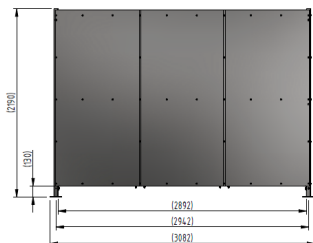
GALVANISED STEEL FRAME AND SIDE PANELS
