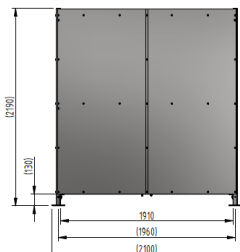
GALVANISED STEEL FRAME AND SIDE PANELS
